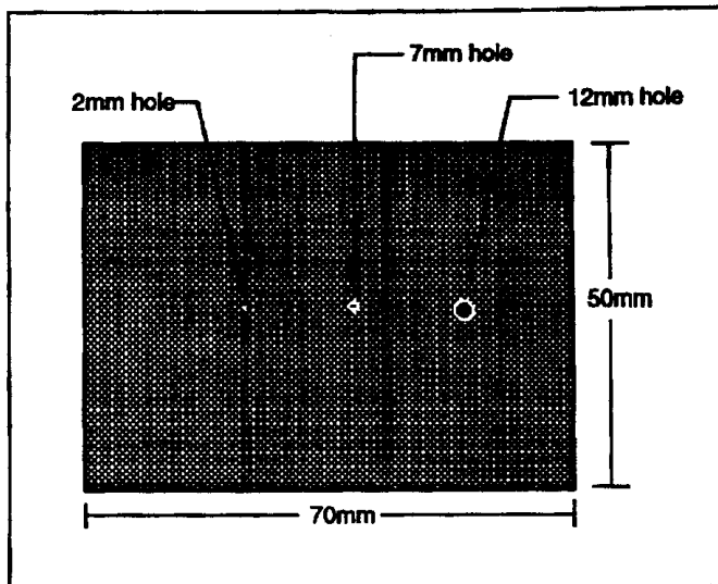
Figure 2. Plate Structure Showing Holes to Scale
