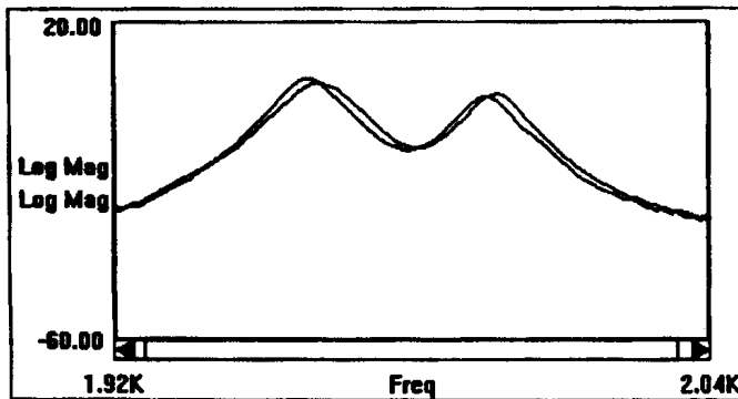
Figure 4.C. Two Modal Peaks of Aluminum Plate Without/With 12mm Hole.
