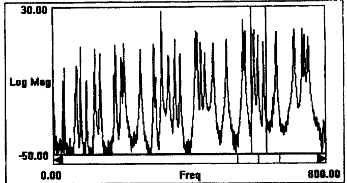
Figure 5. Modal Peaks of Steel Plate With No Hole.
