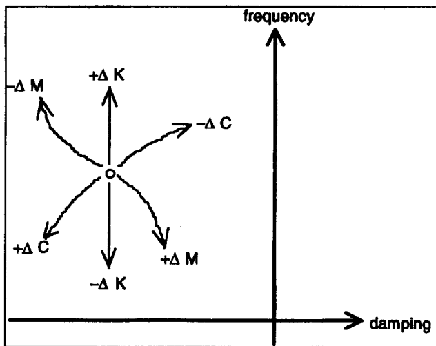
Figure 1. Movement of a Pole Due to Mass, Stiffness, & Damping Changes
