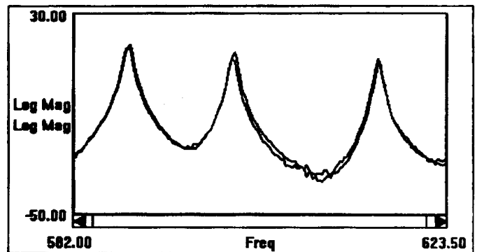
Figure 6.B. Three Modal Peaks of Steel Plate Without/With 7mm Hole.
