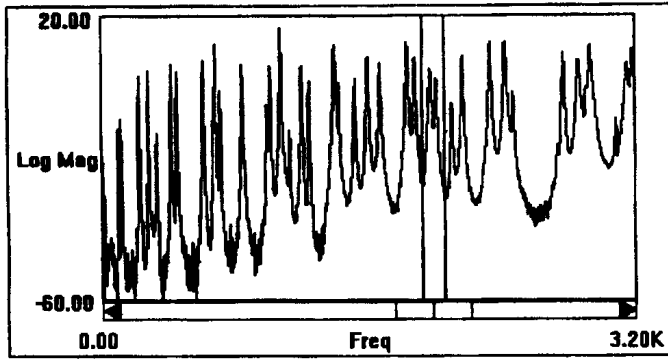
Figure 3. Modal Peaks for Aluminum Plate With No Hole.
