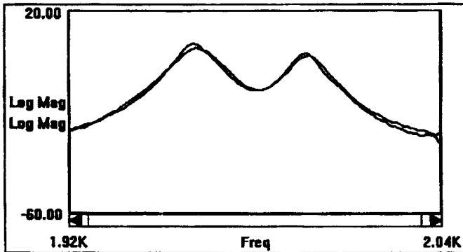
Figure 4.B. Two Modal Peaks of Aluminum Plate Without/With 7mm Hole.
