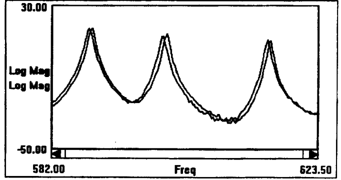
Figure 6.C. Three Modal Peaks of Steel Plate Without/With 12mm Hole.
