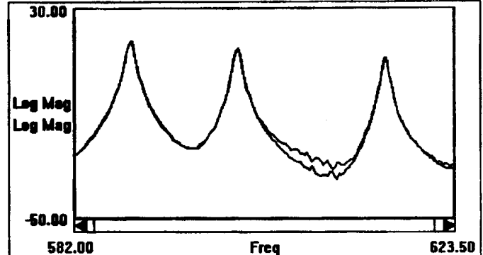
Figure 6.A. Three Modal Peaks of Steel Plate Without/With 2mm Hole.
